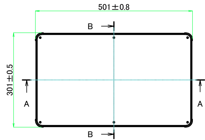
E view
