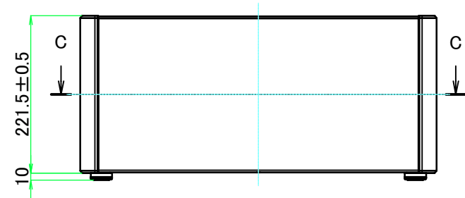
A view
